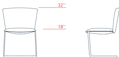
Visitors low-backrest chair, cantilever base 1VE2010 L 22 1/2 P 21 3/4 H 32"
